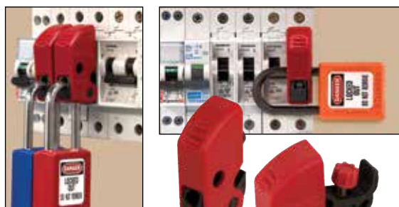
S2394 Side-by-Side Application
